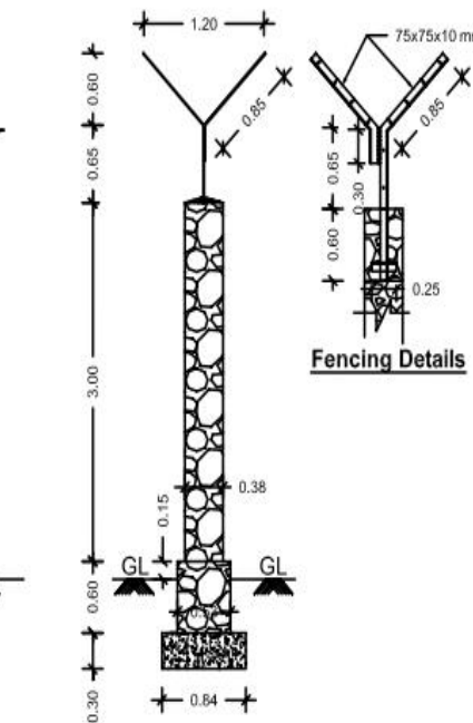
CROSS SECTION
